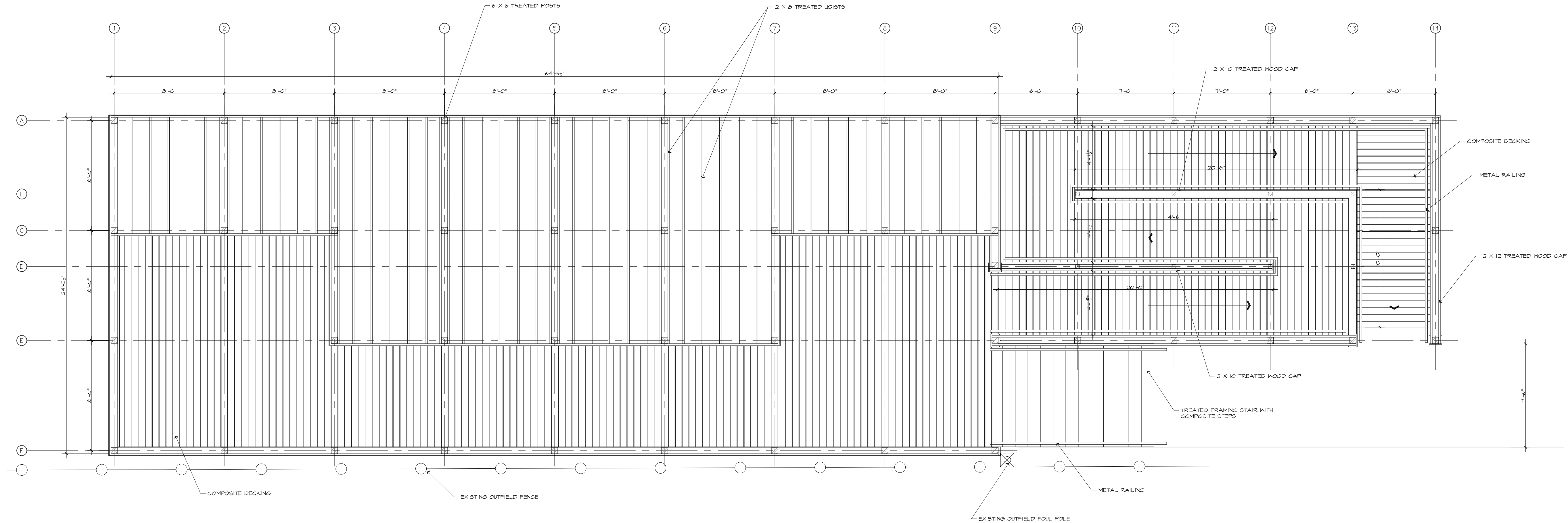
UPPER LEVEL FRAMING PLAN SCALE: 1/4"=1'-0"
