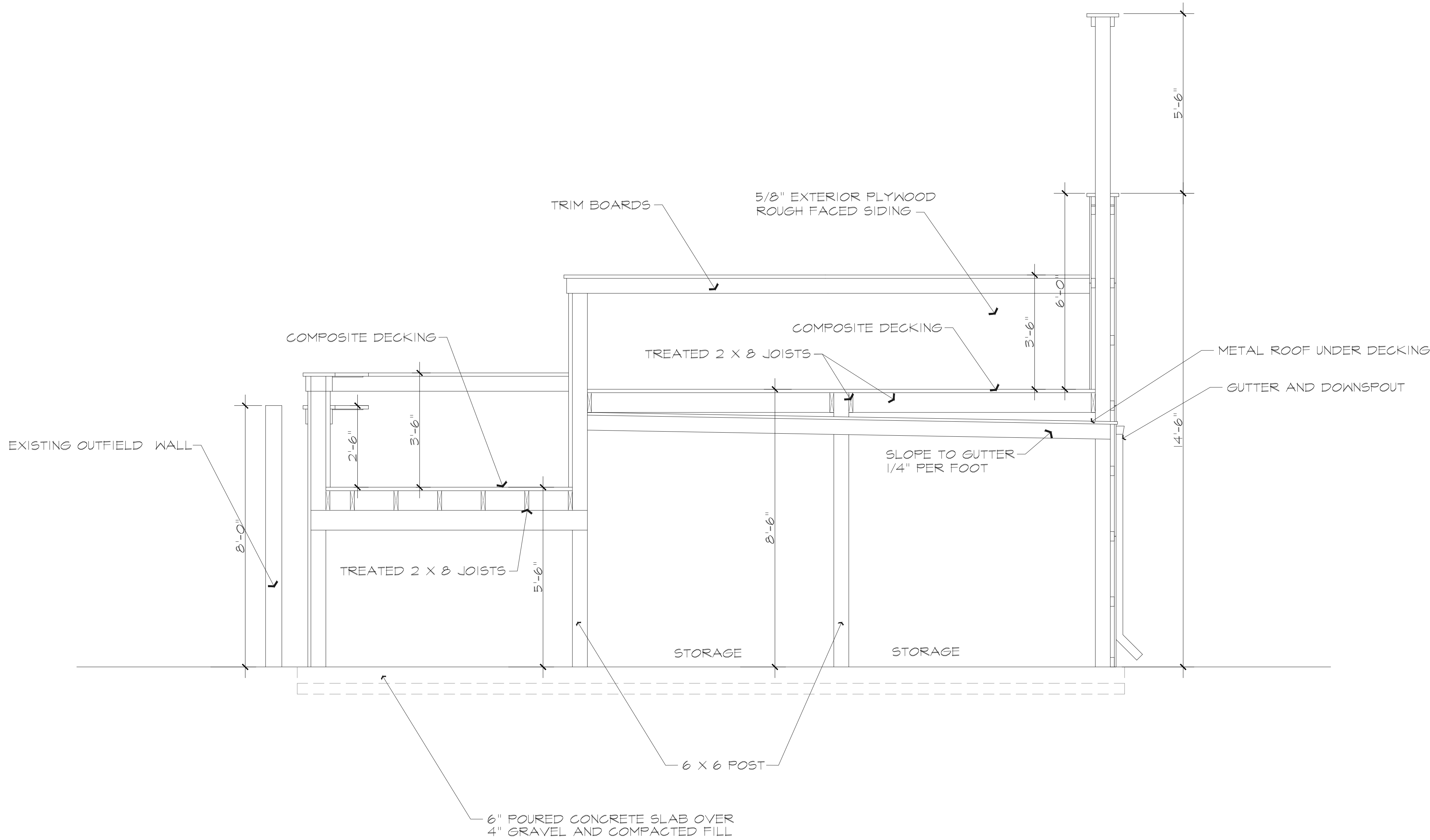
BUILDING SECTION I SCALE: 1/2"=1'-0"
